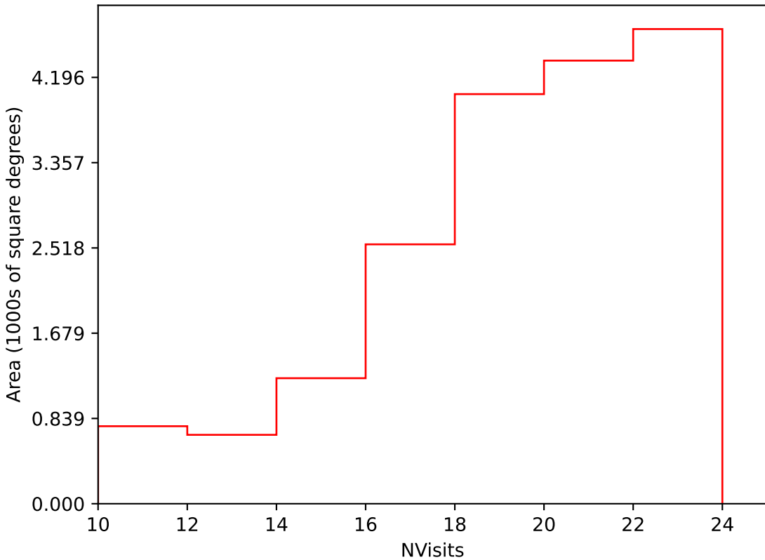
too_elab_r64_d3_ugrizy_v3.4_10yrs Yr 1 i band: NVisits
