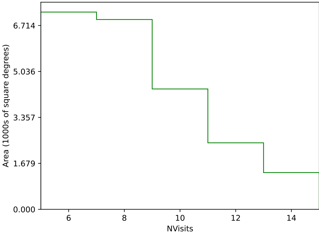
too_elab_r64_d3_ugrizy_v3.4_10yrs Yr 1 g band: NVisits
