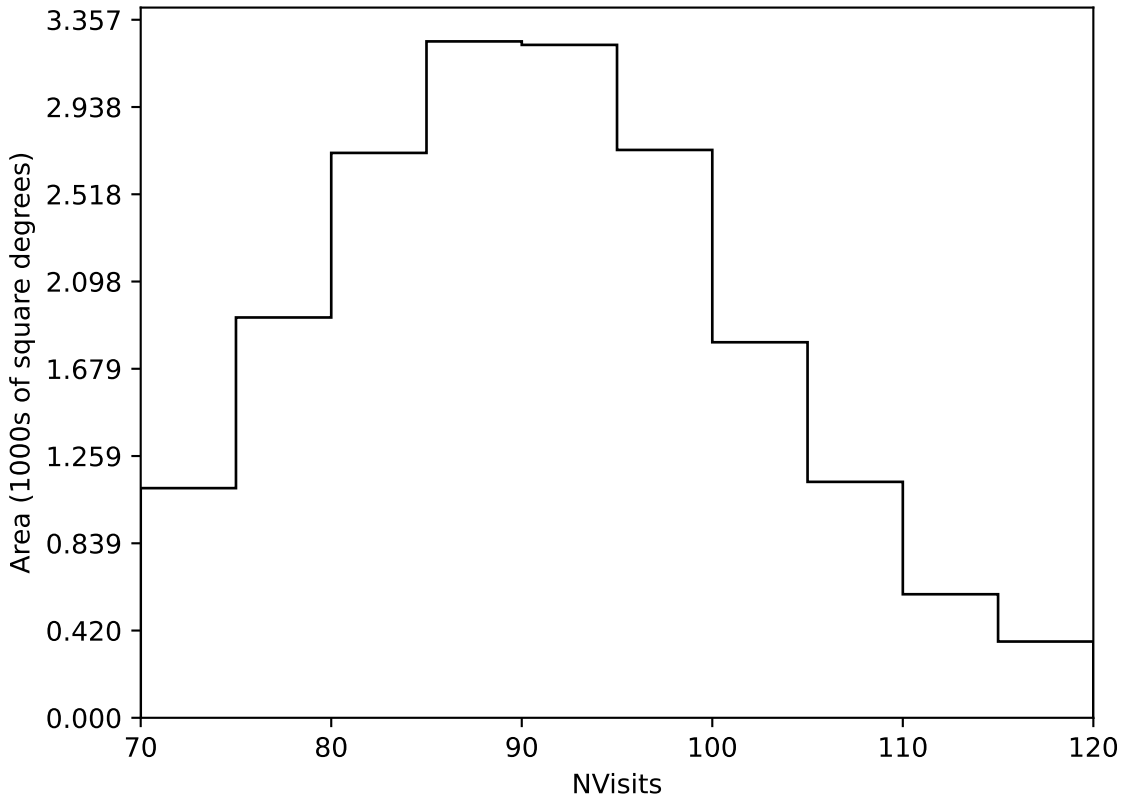
too_elab_r64_d3_ugrizy_v3.4_10yrs Yr 1 all bands: NVisits
