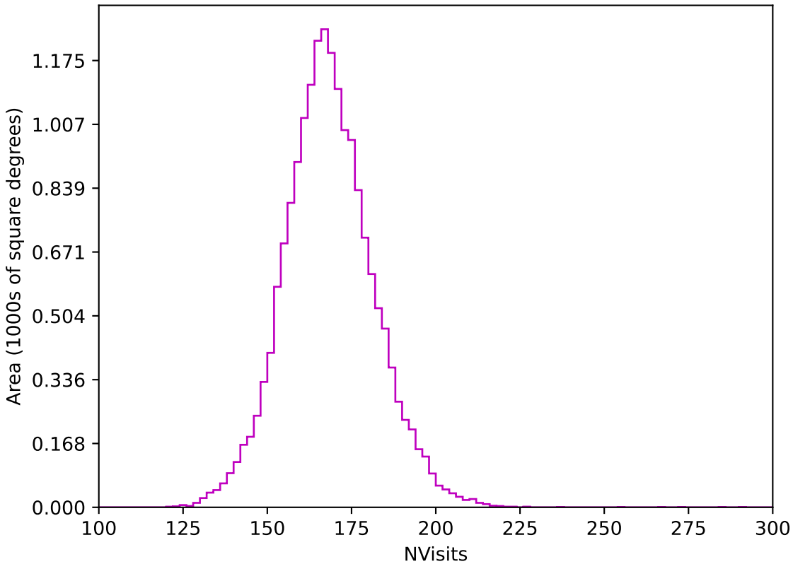
too_elab_r64_d3_ugrizy_v3.4_10yrs WFD z band: NVisits
