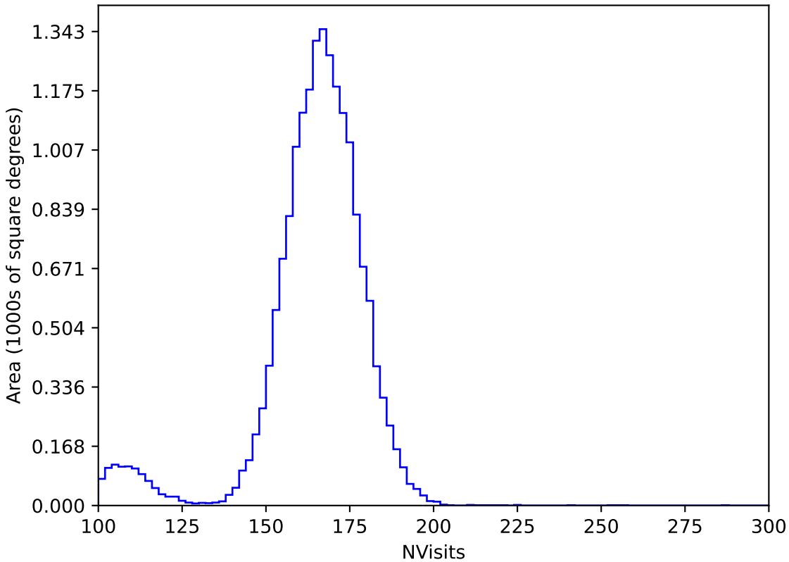
too_elab_r64_d3_ugrizy_v3.4_10yrs WFD y band: NVisits
