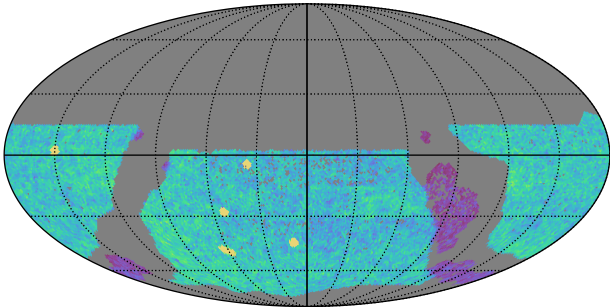
too_elab_r64_d3_ugrizy_v3.4_10yrs WFD u band: NVisits
