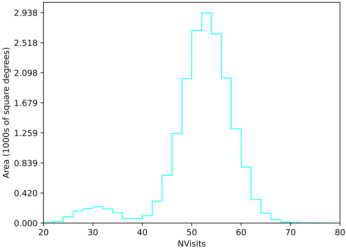
too_elab_r64_d3_ugrizy_v3.4_10yrs WFD u band: NVisits
