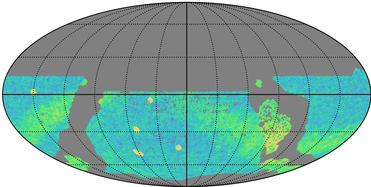
too_elab_r64_d3_ugrizy_v3.4_10yrs WFD r band: NVisits
