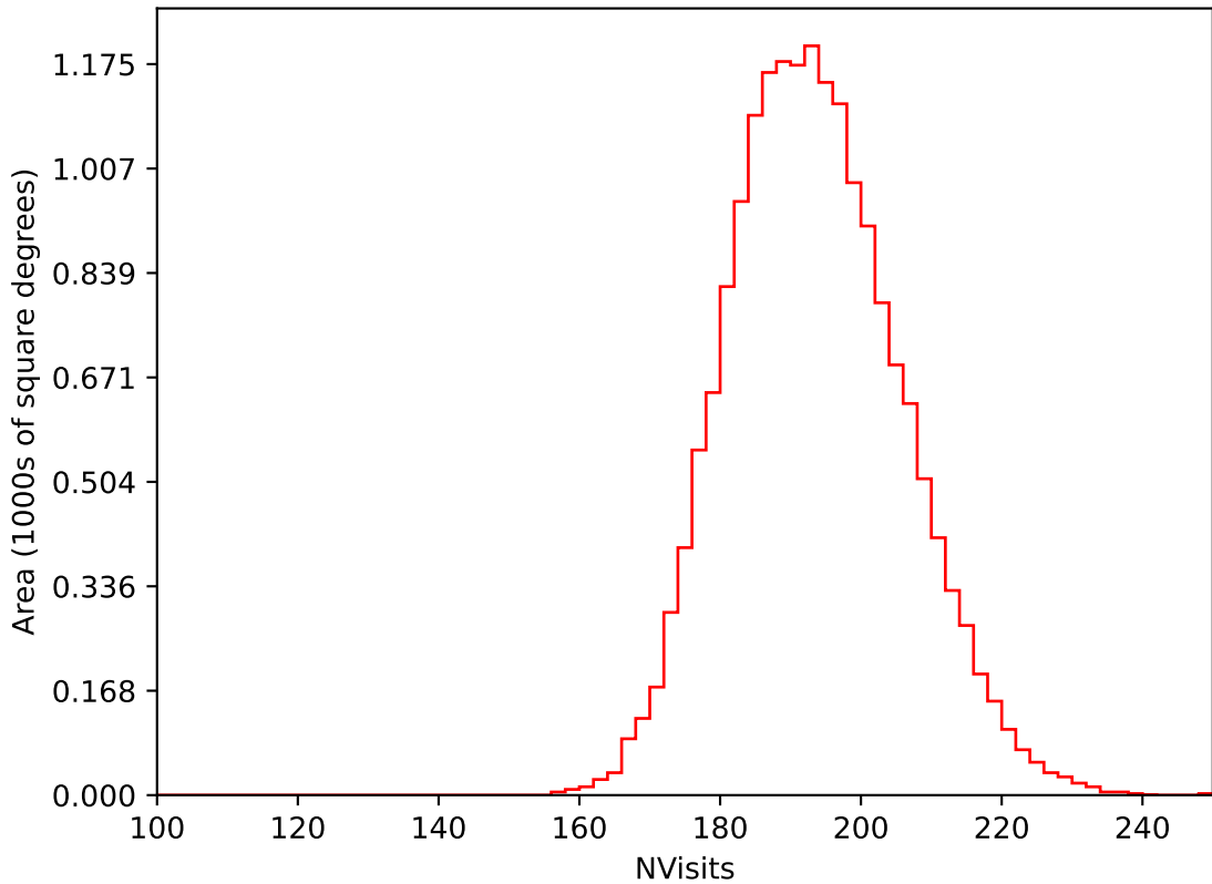
too_elab_r64_d3_ugrizy_v3.4_10yrs WFD i band: NVisits
