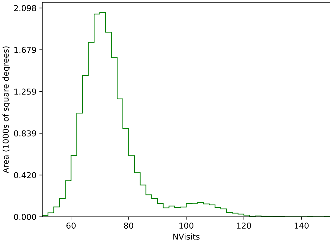
too_elab_r64_d3_ugrizy_v3.4_10yrs WFD g band: NVisits
