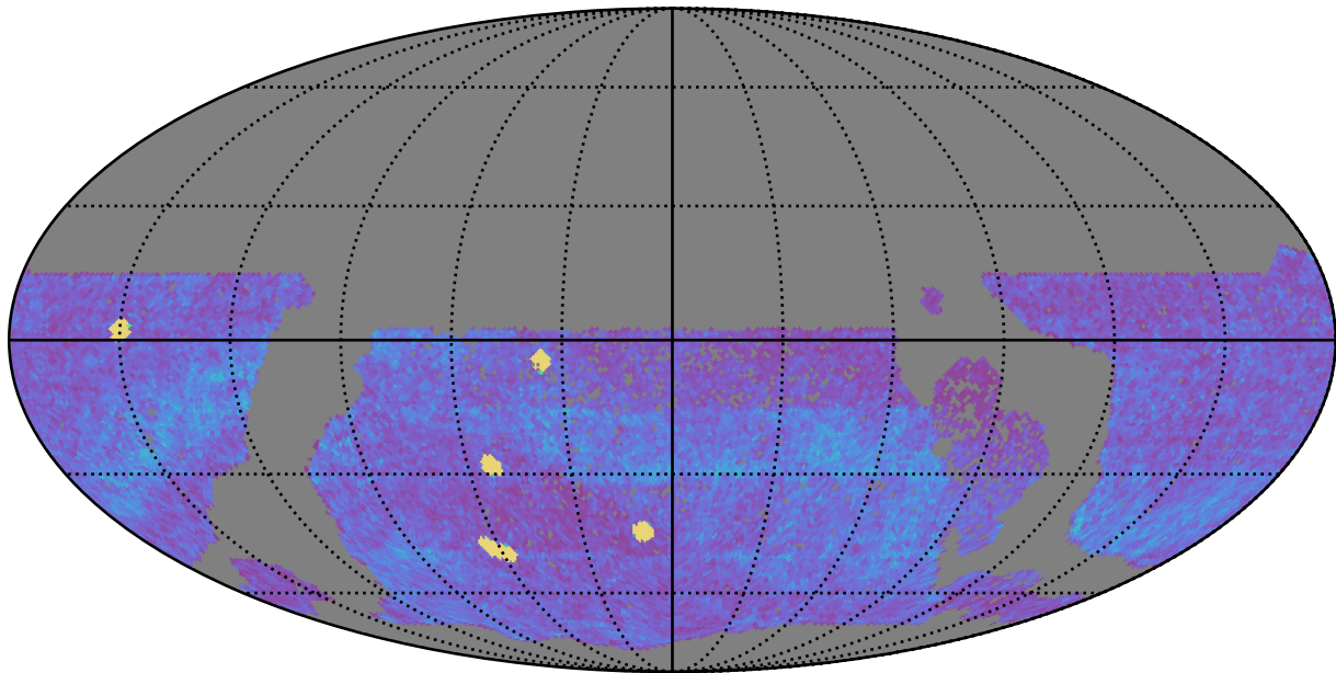
too_elab_r64_d3_ugrizy_v3.4_10yrs WFD all bands: NVisits
