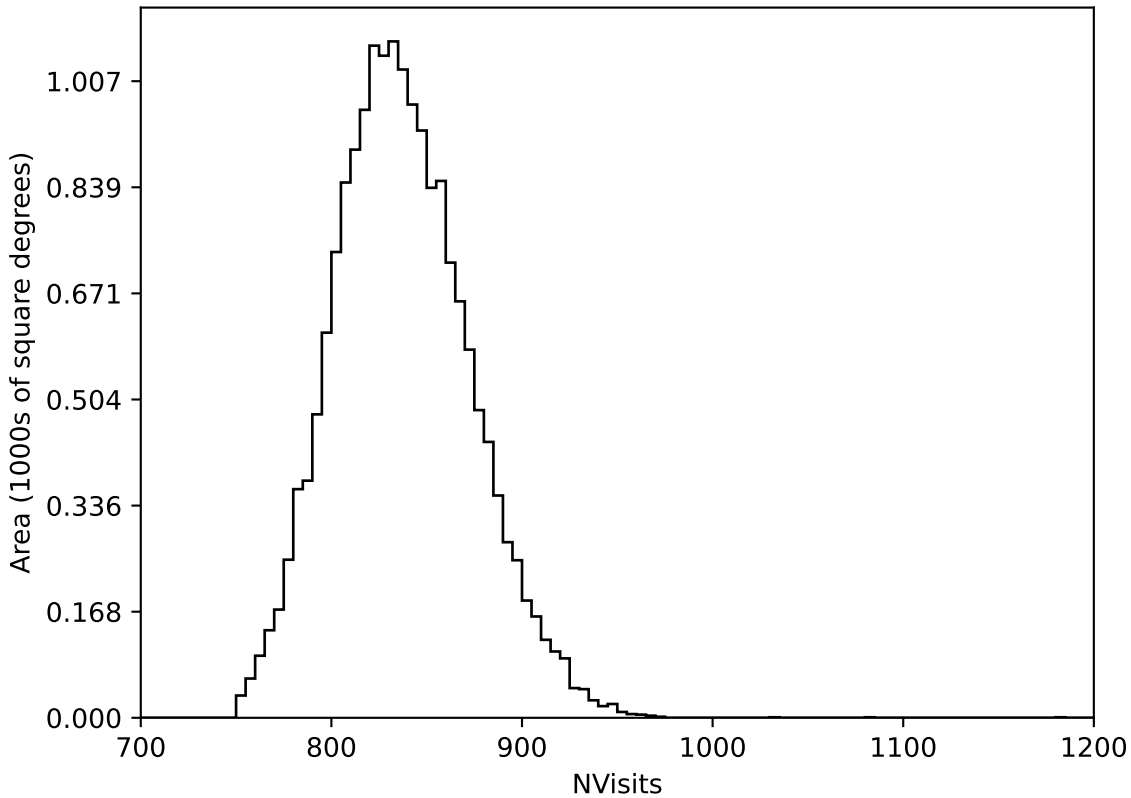
too_elab_r64_d3_ugrizy_v3.4_10yrs WFD all bands: NVisits
