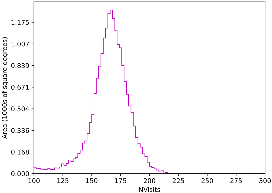
too_elab_r64_d3_ugrizy_v3.4_10yrs All sky z band: NVisits
