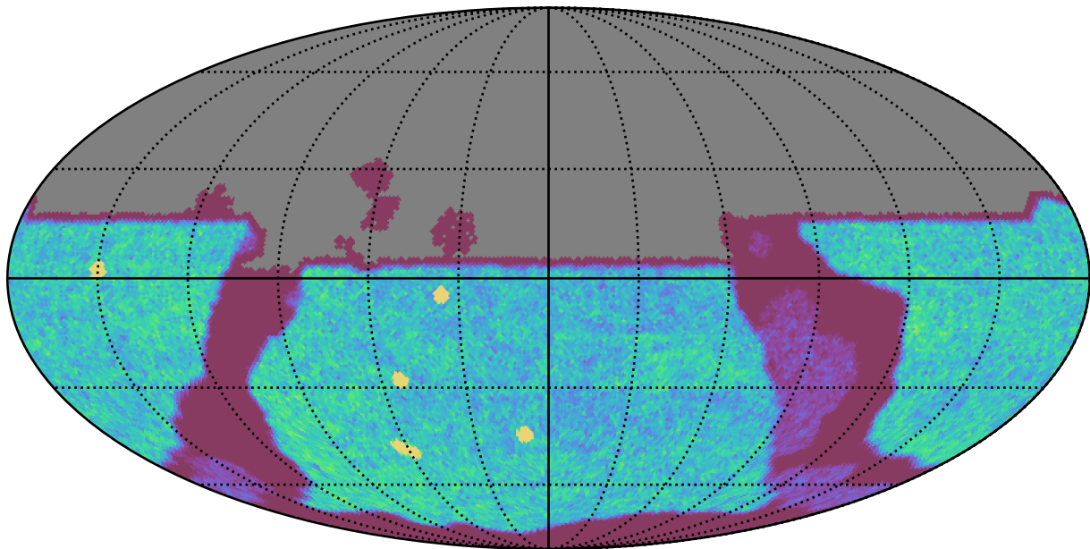
too_elab_r64_d3_ugrizy_v3.4_10yrs All sky u band: NVisits
