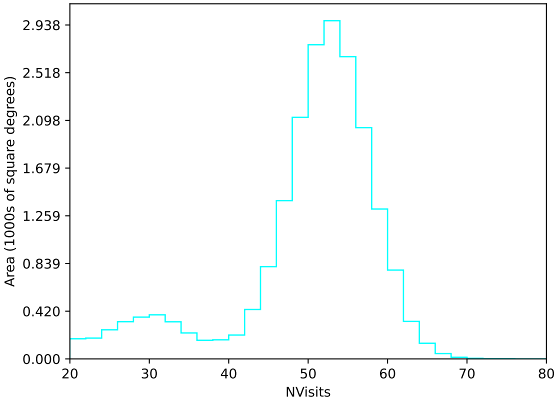
too_elab_r64_d3_ugrizy_v3.4_10yrs All sky u band: NVisits
