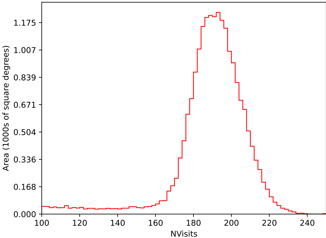
too_elab_r64_d3_ugrizy_v3.4_10yrs All sky i band: NVisits
