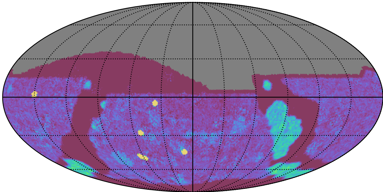
too_elab_r64_d3_ugrizy_v3.4_10yrs All sky g band: NVisits
