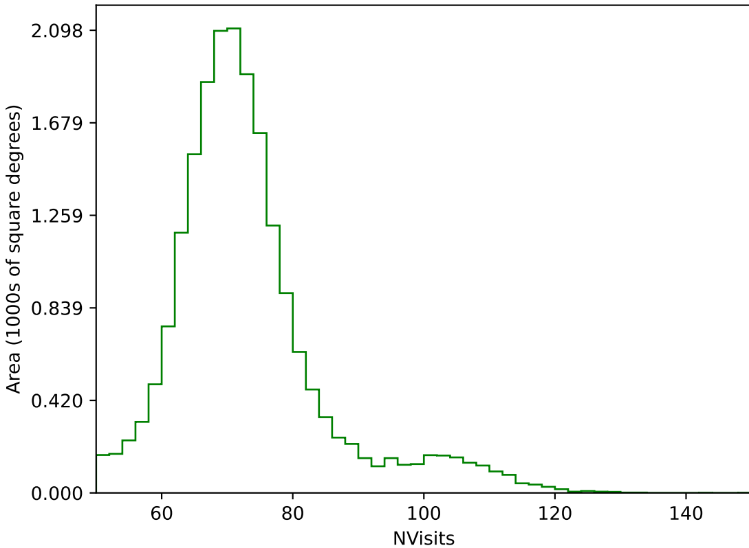
too_elab_r64_d3_ugrizy_v3.4_10yrs All sky g band: NVisits
