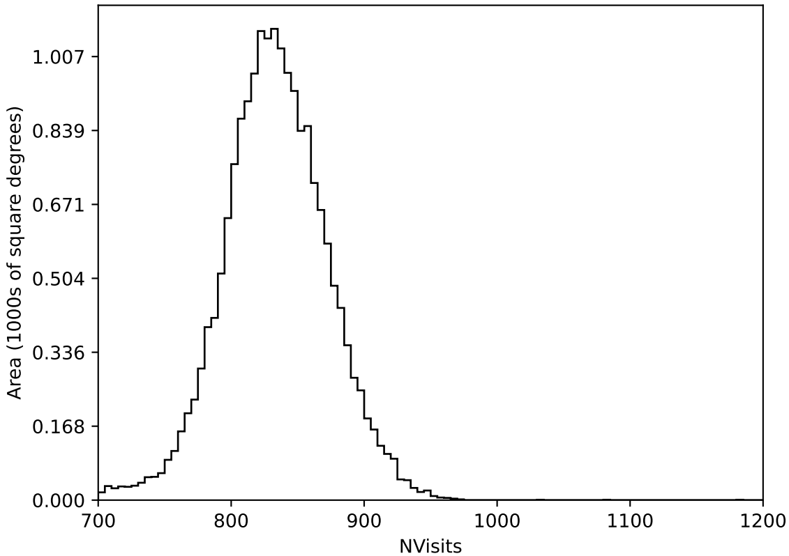
too_elab_r64_d3_ugrizy_v3.4_10yrs All sky all bands: NVisits
