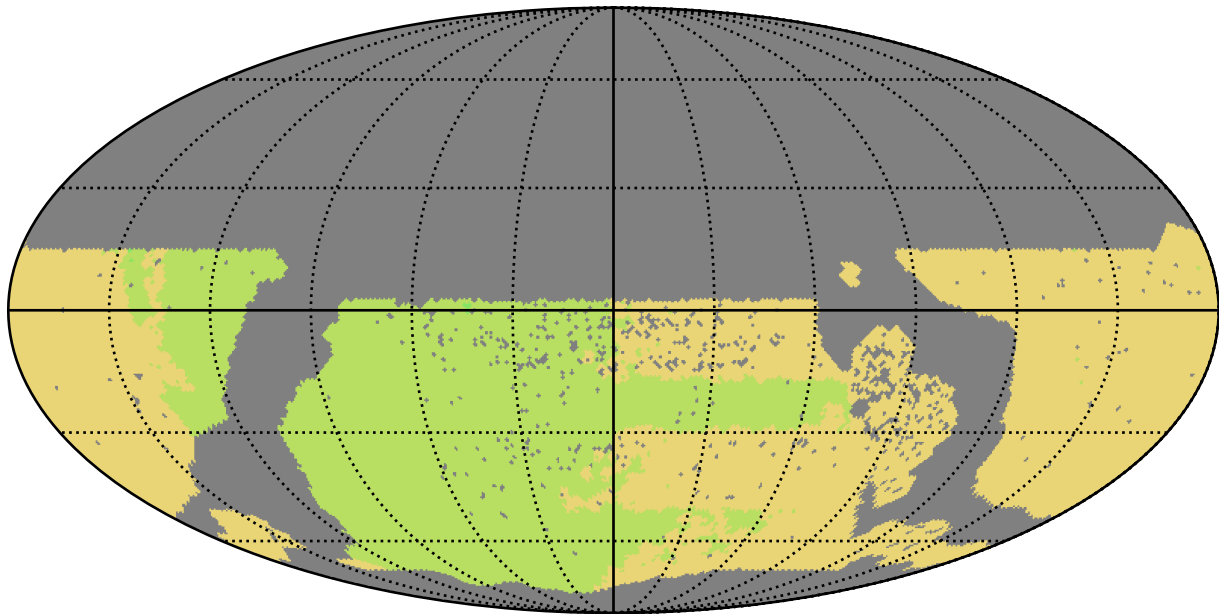
too_elab_r64_d3_ugrizy_v3.4_10yrs WFD all bands: NSeasons
