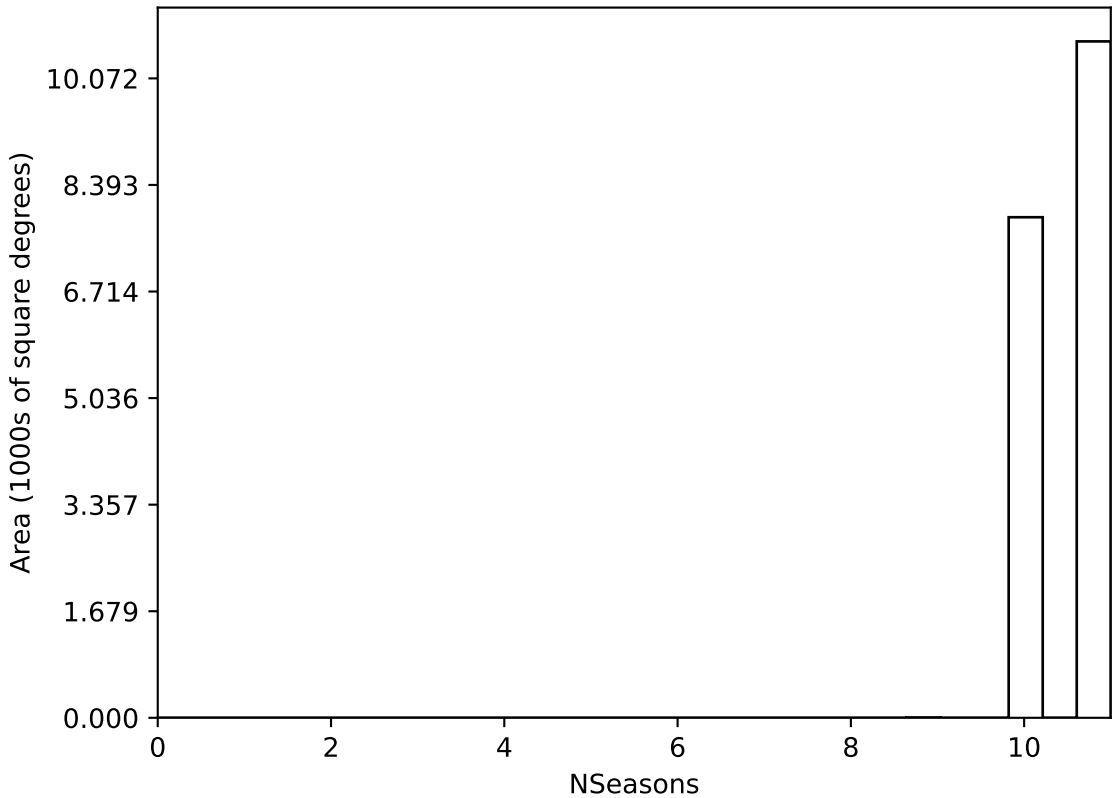
too_elab_r64_d3_ugrizy_v3.4_10yrs WFD all bands: NSeasons
