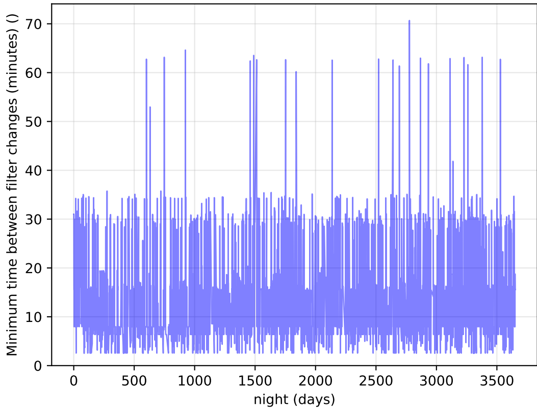
too_elab_r64_d3_ugrizy_v3.4_10yrs Per Night: Minimum time between filter changes (minutes)
