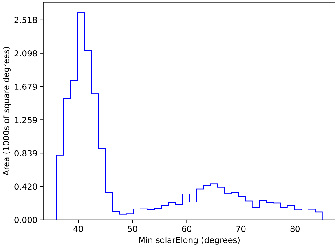
too_elab_r64_d3_ugrizy_v3.4_10yrs WFD z band: Min solarElong
