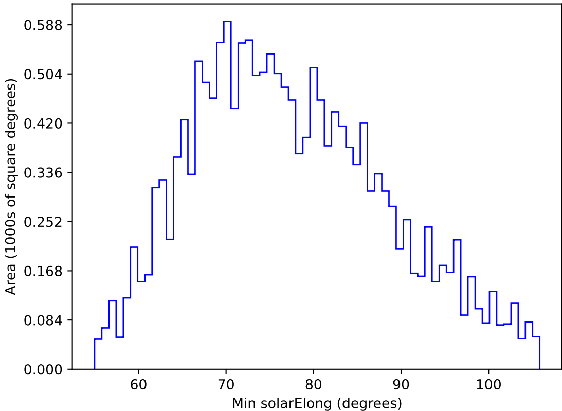
too_elab_r64_d3_ugrizy_v3.4_10yrs WFD u band: Min solarElong
