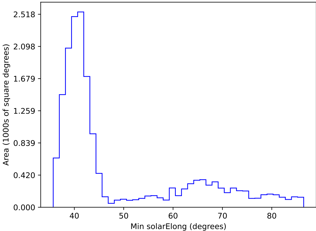
too_elab_r64_d3_ugrizy_v3.4_10yrs WFD i band: Min solarElong
