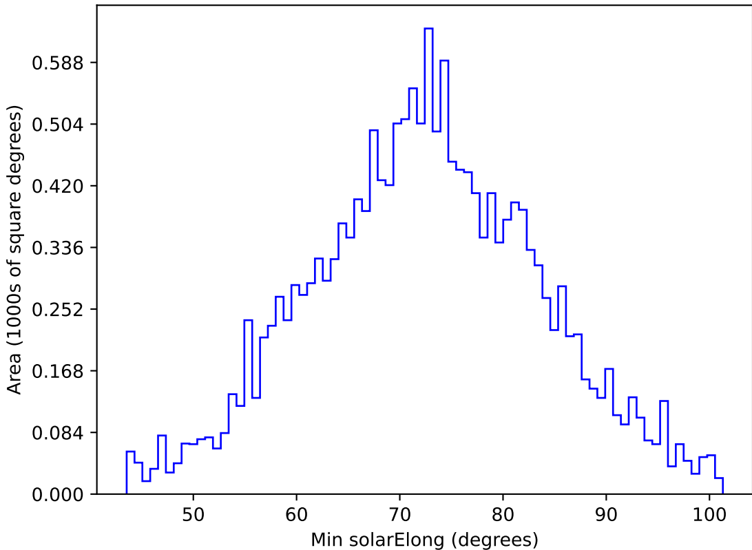
too_elab_r64_d3_ugrizy_v3.4_10yrs WFD g band: Min solarElong
