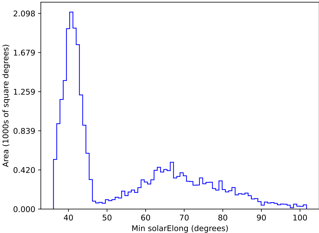
too_elab_r64_d3_ugrizy_v3.4_10yrs All sky z band: Min solarElong
