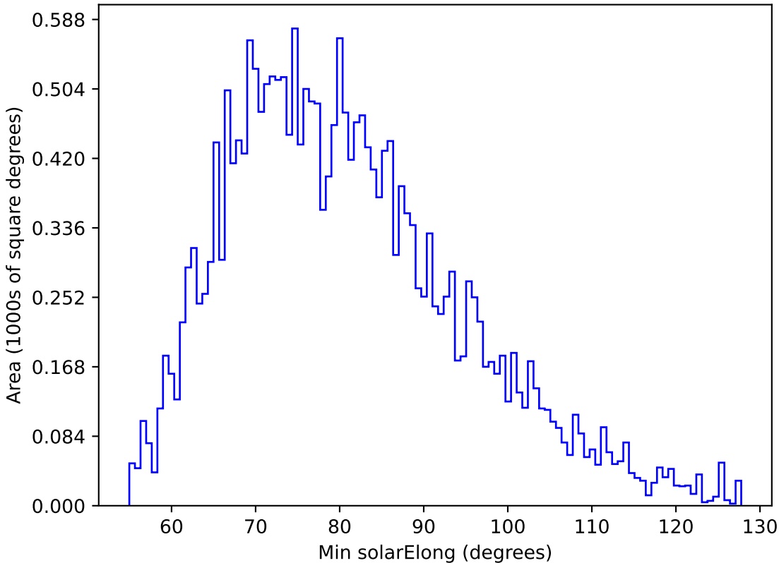
too_elab_r64_d3_ugrizy_v3.4_10yrs All sky u band: Min solarElong
