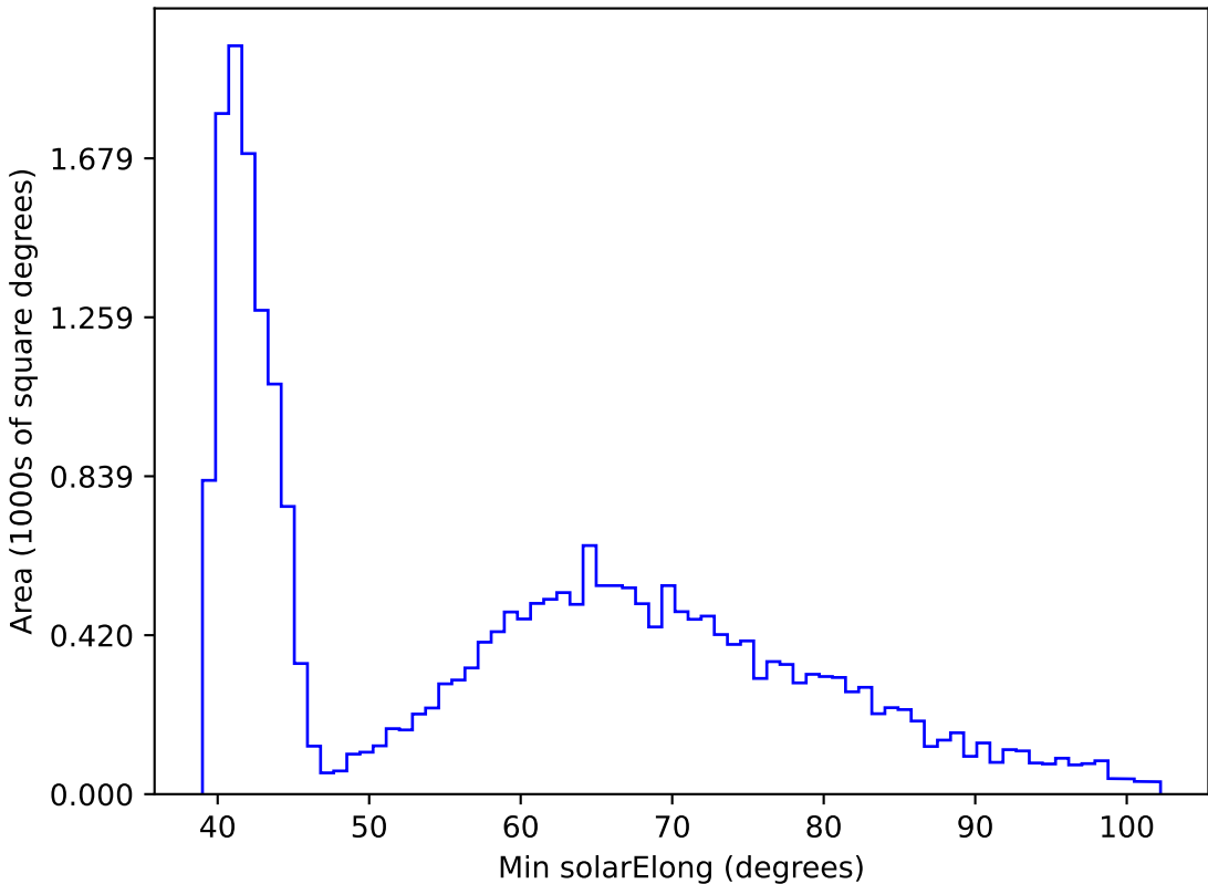
too_elab_r64_d3_ugrizy_v3.4_10yrs All sky r band: Min solarElong
