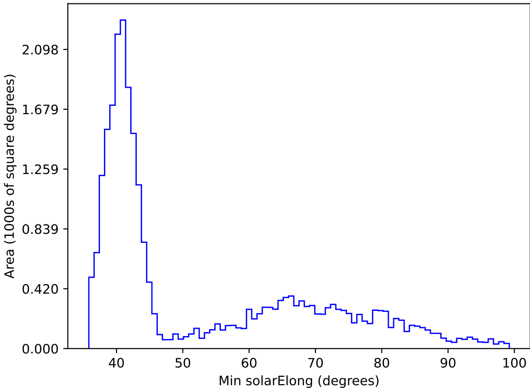
too_elab_r64_d3_ugrizy_v3.4_10yrs All sky i band: Min solarElong
