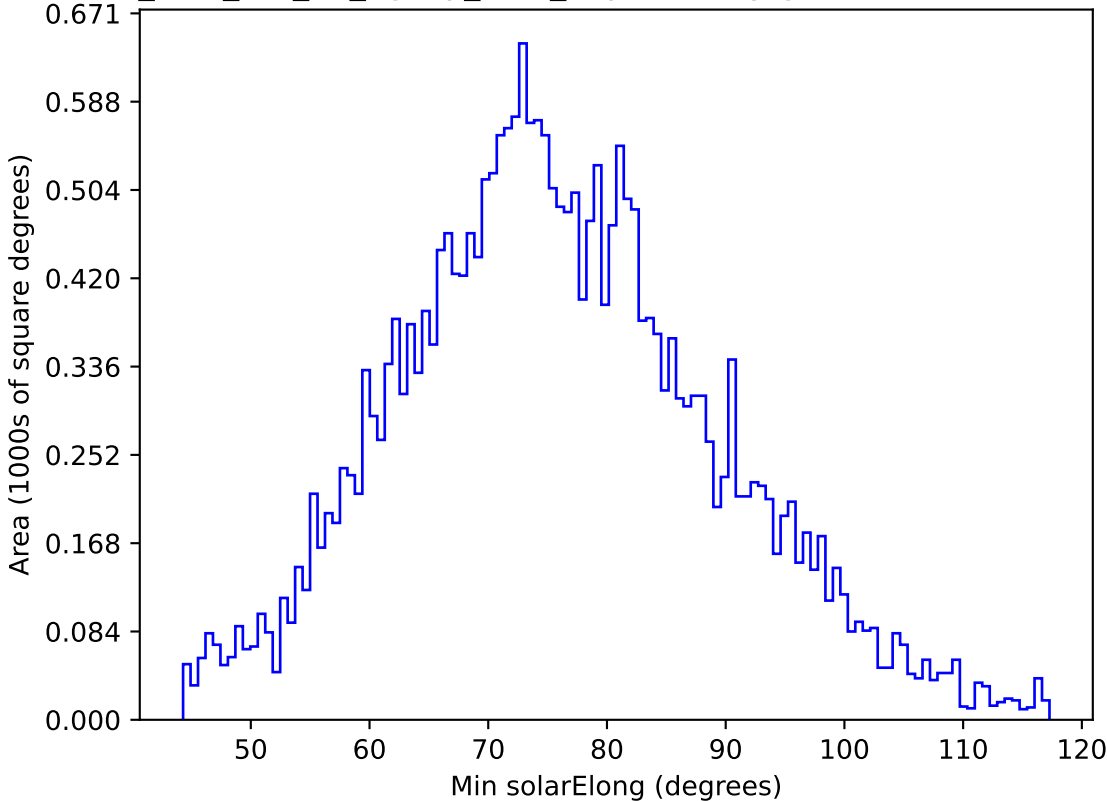
too_elab_r64_d3_ugrizy_v3.4_10yrs All sky g band: Min solarElong
