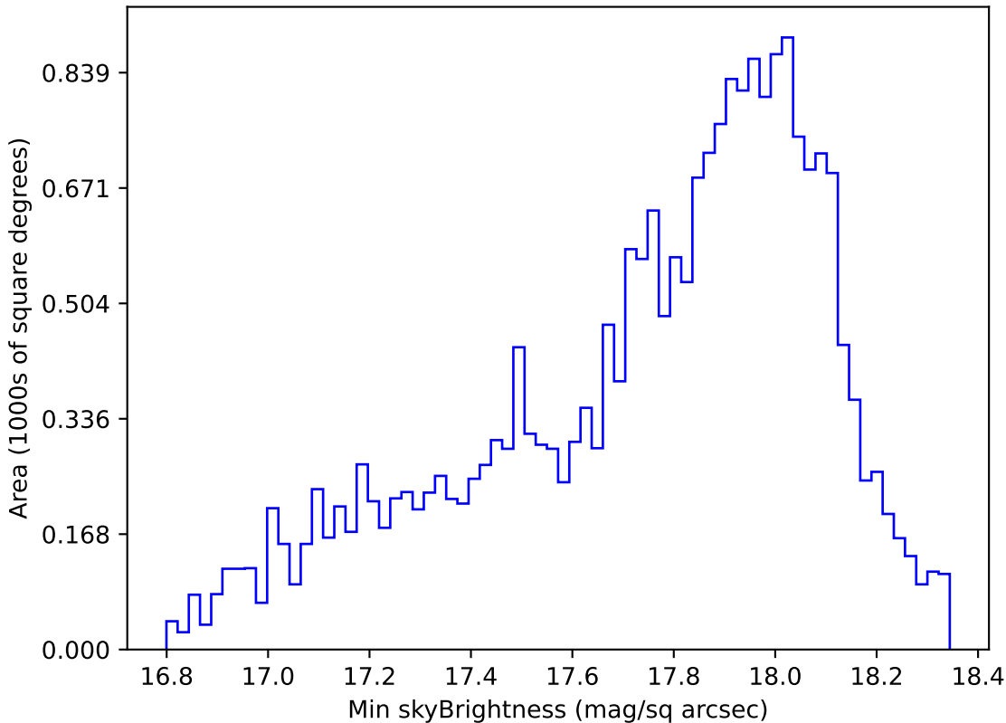
too_elab_r64_d3_ugrizy_v3.4_10yrs Yr 1 y band: Min skyBrightness
