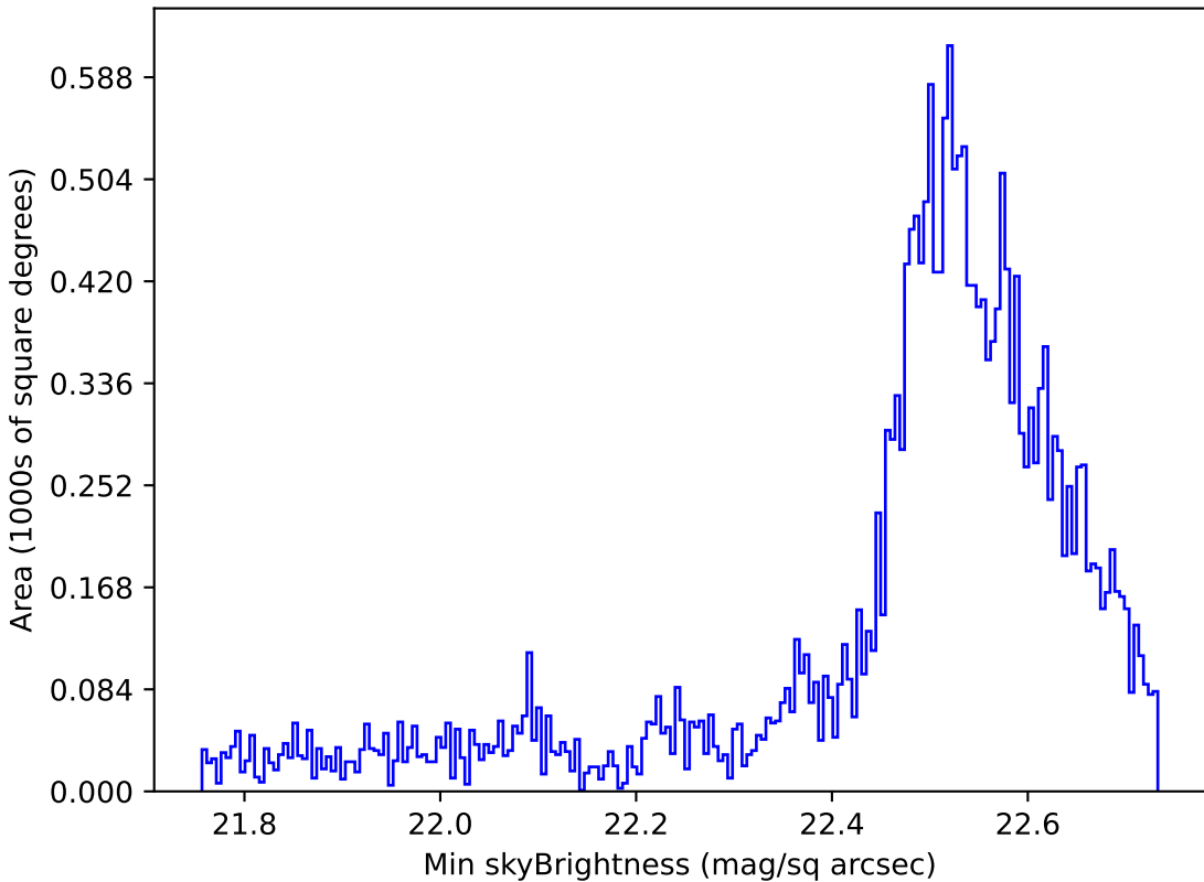
too_elab_r64_d3_ugrizy_v3.4_10yrs Yr 1 u band: Min skyBrightness
