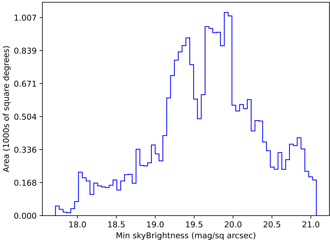
too_elab_r64_d3_ugrizy_v3.4_10yrs Yr 1 r band: Min skyBrightness
