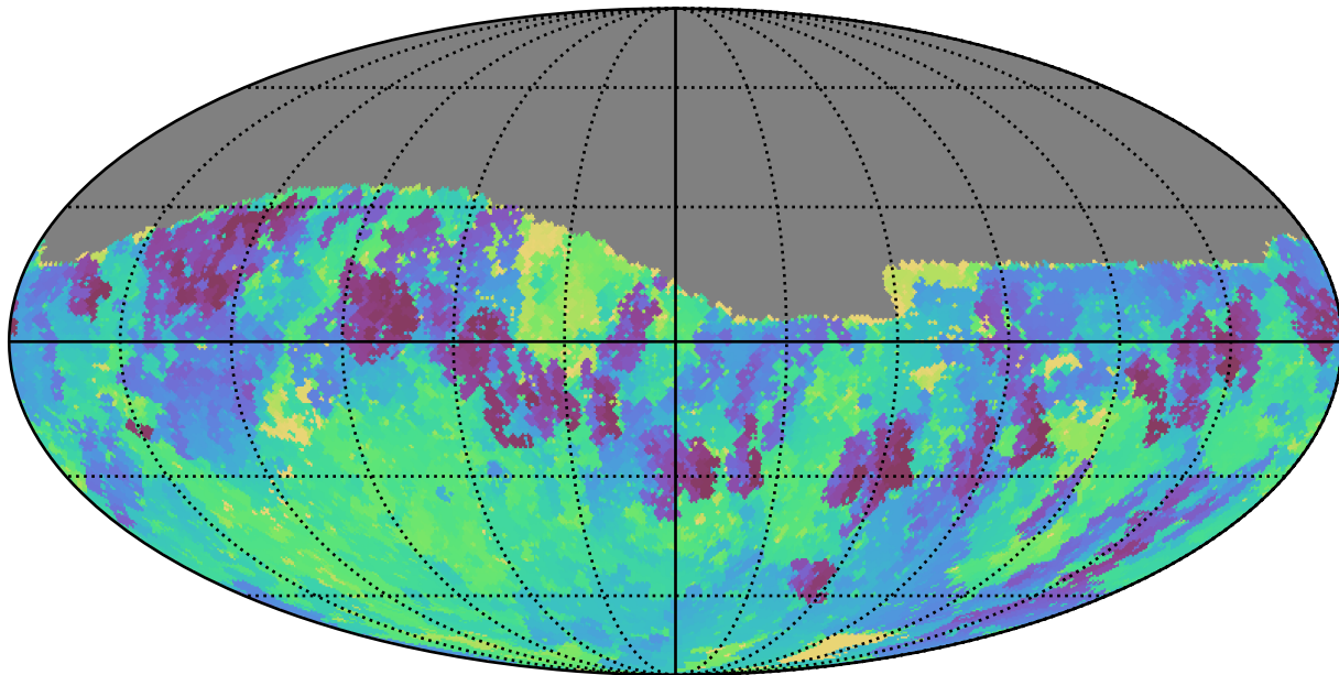
too_elab_r64_d3_ugrizy_v3.4_10yrs Yr 1 i band: Min skyBrightness
