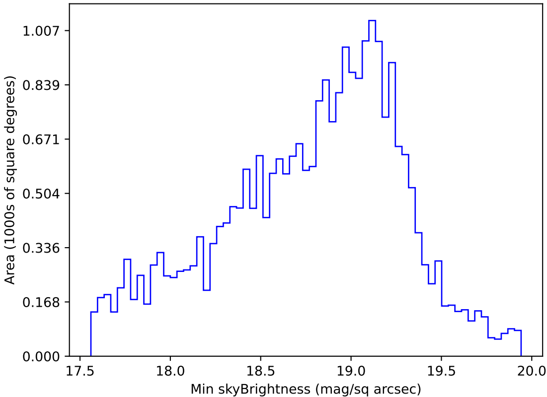
too_elab_r64_d3_ugrizy_v3.4_10yrs Yr 1 i band: Min skyBrightness
