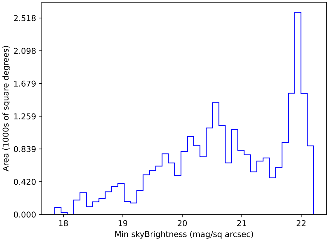
too_elab_r64_d3_ugrizy_v3.4_10yrs Yr 1 g band: Min skyBrightness
