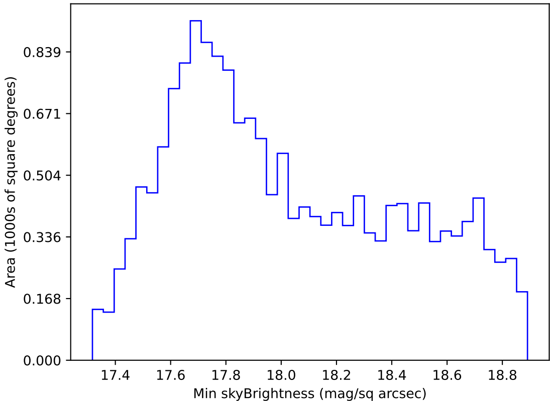
too_elab_r64_d3_ugrizy_v3.4_10yrs WFD i band: Min skyBrightness
