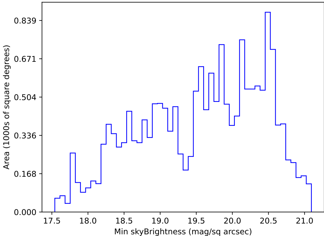
too_elab_r64_d3_ugrizy_v3.4_10yrs WFD g band: Min skyBrightness
