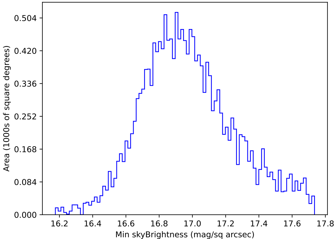
too_elab_r64_d3_ugrizy_v3.4_10yrs WFD all bands: Min skyBrightness
