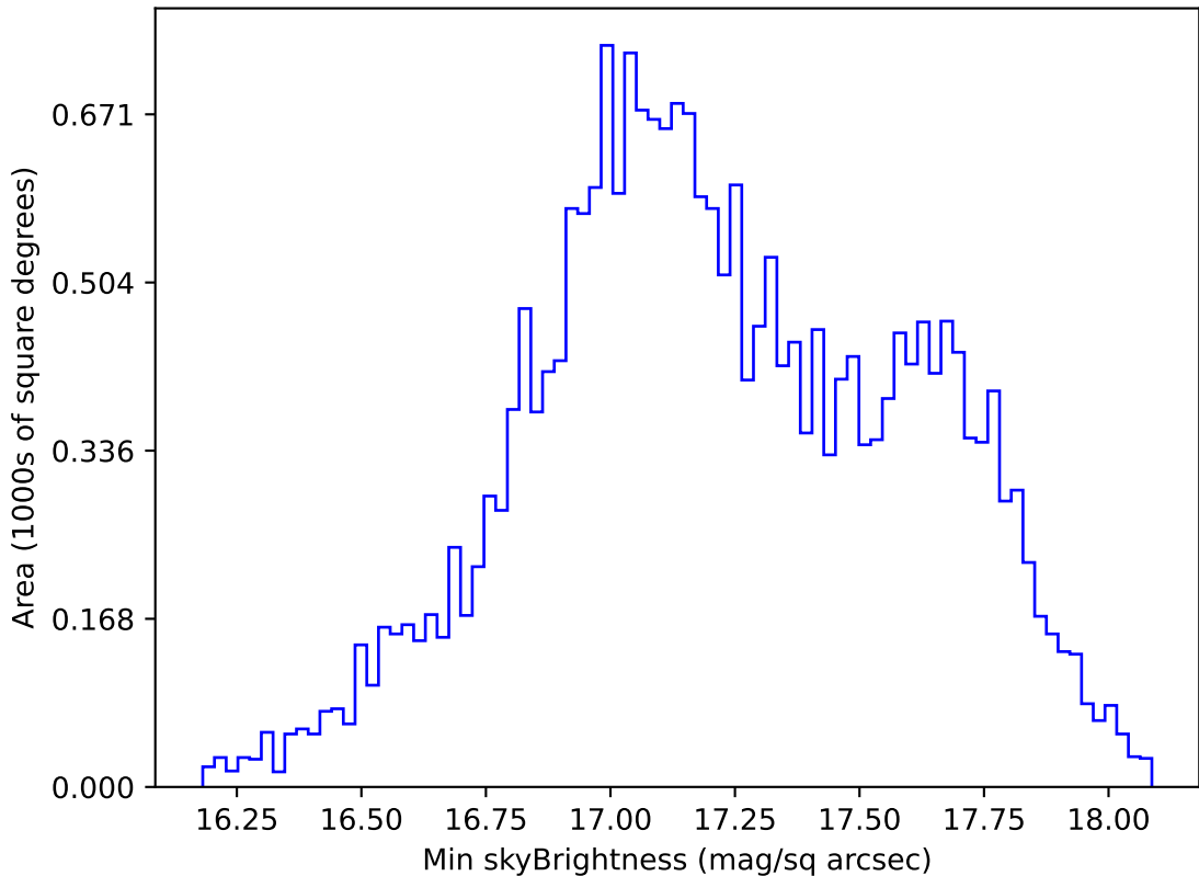
too_elab_r64_d3_ugrizy_v3.4_10yrs All sky y band: Min skyBrightness
