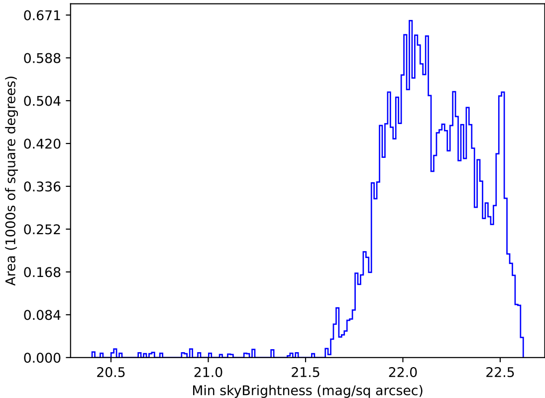
too_elab_r64_d3_ugrizy_v3.4_10yrs All sky u band: Min skyBrightness
