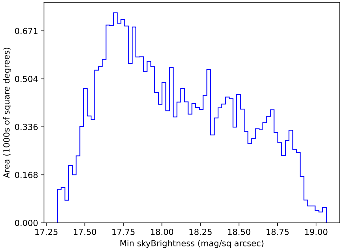
too_elab_r64_d3_ugrizy_v3.4_10yrs All sky i band: Min skyBrightness
