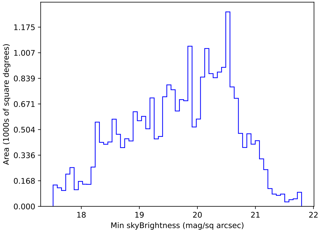
too_elab_r64_d3_ugrizy_v3.4_10yrs All sky g band: Min skyBrightness
