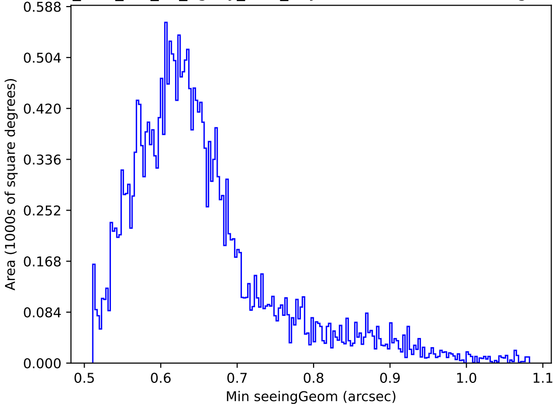
too_elab_r64_d3_ugrizy_v3.4_10yrs Yr 1 z band: Min seeingGeom
