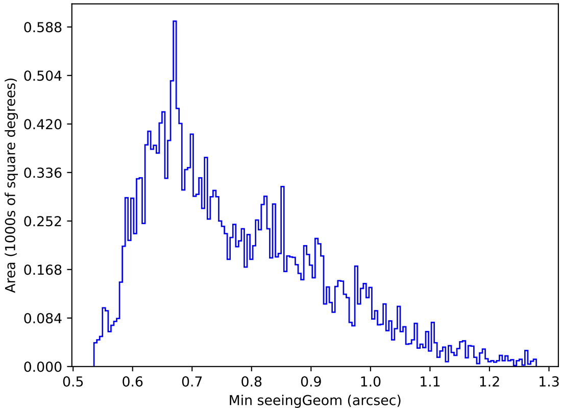
too_elab_r64_d3_ugrizy_v3.4_10yrs Yr 1 u band: Min seeingGeom
