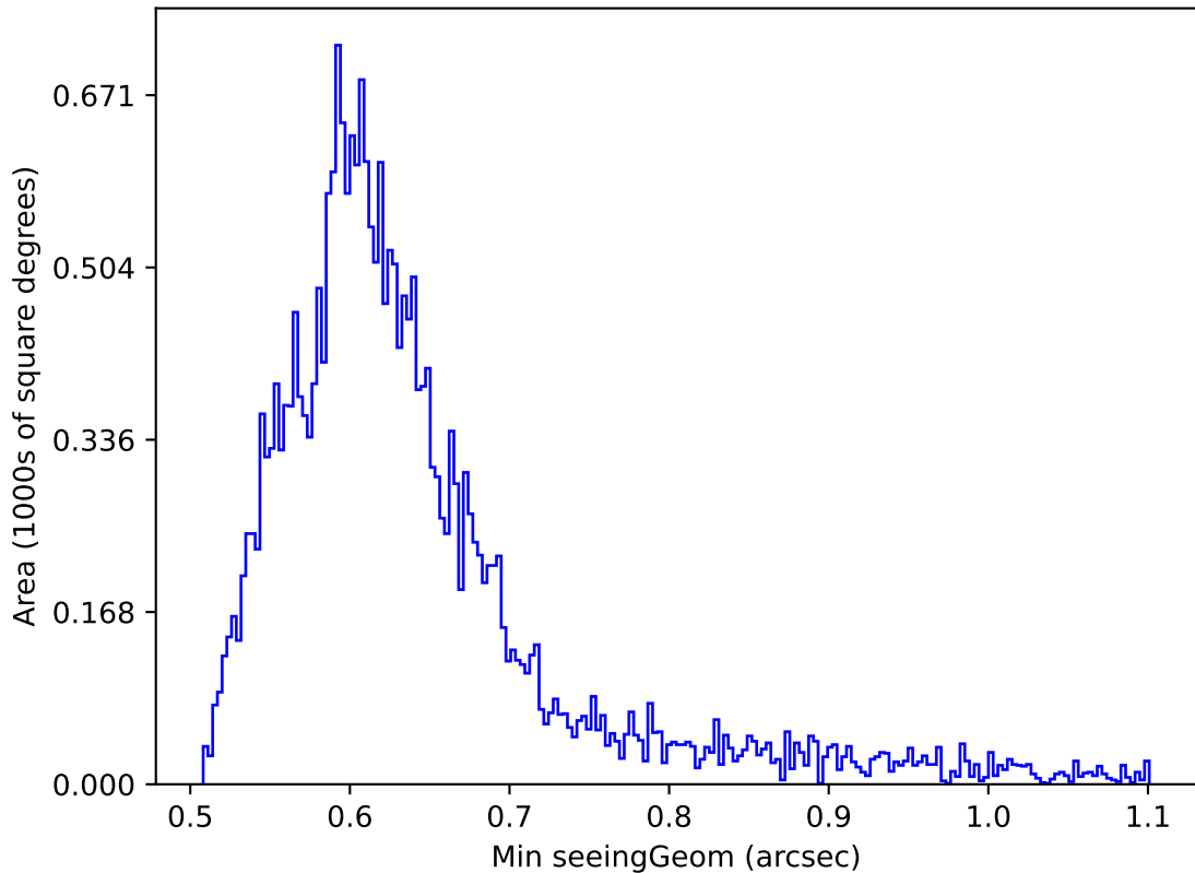
too_elab_r64_d3_ugrizy_v3.4_10yrs Yr 1 r band: Min seeingGeom
