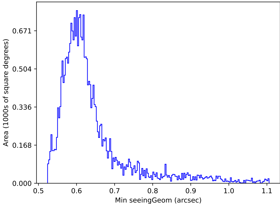
too_elab_r64_d3_ugrizy_v3.4_10yrs Yr 1 i band: Min seeingGeom
