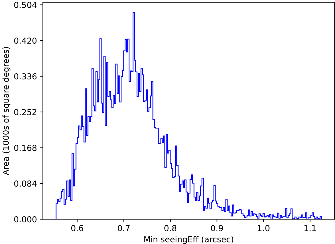
too_elab_r64_d3_ugrizy_v3.4_10yrs Yr 1 y band: Min seeingEff
