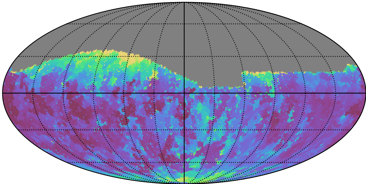
too_elab_r64_d3_ugrizy_v3.4_10yrs Yr 1 g band: Min seeingEff
